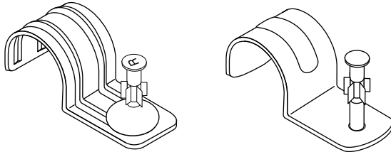
.300 Head Pins with Conduit and BX Cable Straps
